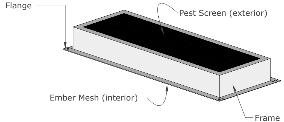
ISOMETRIC VIEW
