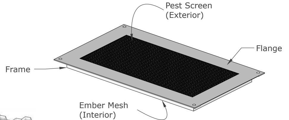
ISOMETRIC VIEW
